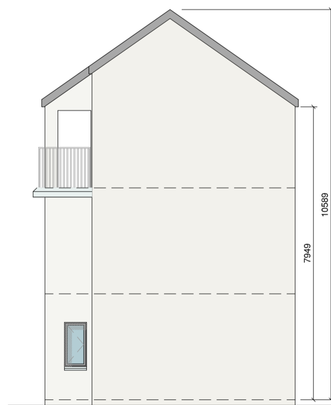
Side Elevation
